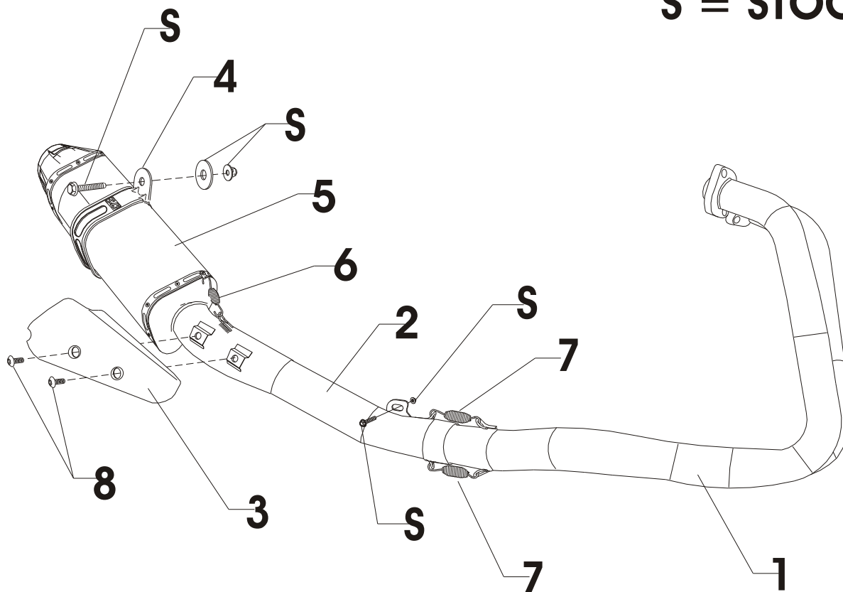
Parts Diagram
