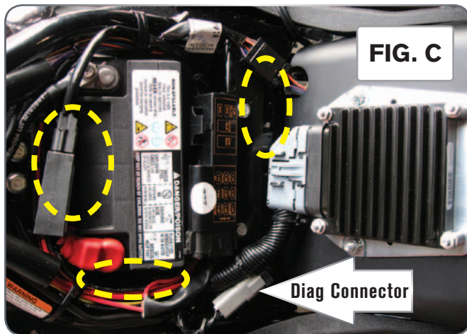
On many Softail models you can typically find a place under the seat to store the module (Fig. C). It could go in the recess at the top of the battery, on the side of the battery, on the relay bracket, or even directly on the rear fender.
