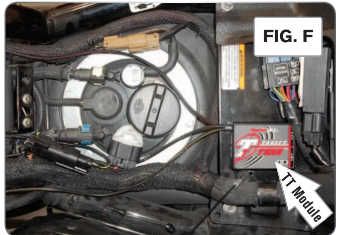
On V-Rod models, the best location to secure the module is directly under the seat (Fig. F).
