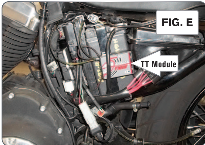
On Sportsters, the left side of the battery is usually the best location to secure the module (Fig. E).
