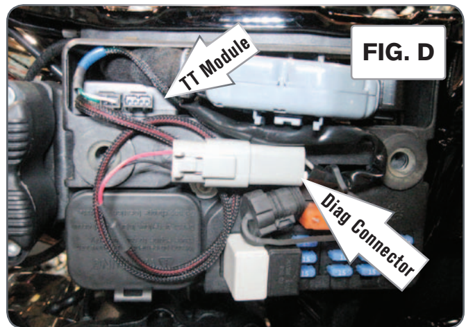
On Dyna models you can typically fit the Target Tune module inside the electrical box next to the ECM (Fig. D).
