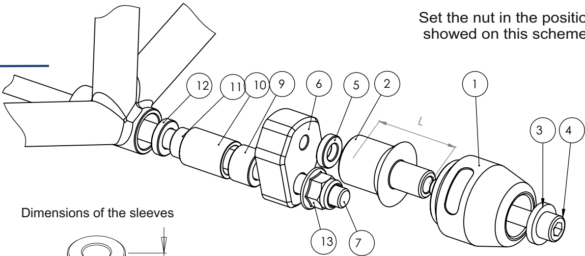
Assembly scheme (both sides)
