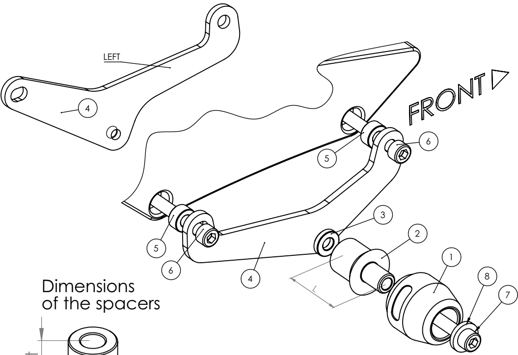
Assembly scheme (both sides)
