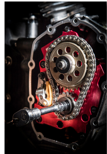
PART #3042
