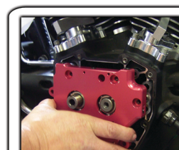
Wiggling assembly while rotating engine back & forth will aid alignment & installation
