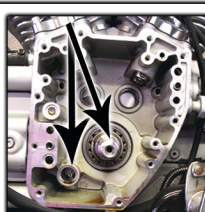
Apply engine assembly lube to camshafts, inner cam bearings, scavenge port hole of case and pick up port of oil pump
