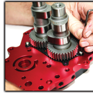
Install bearing retainer plate using loctite
