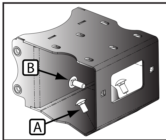
"Figure 6" Carriage Bolt Install
