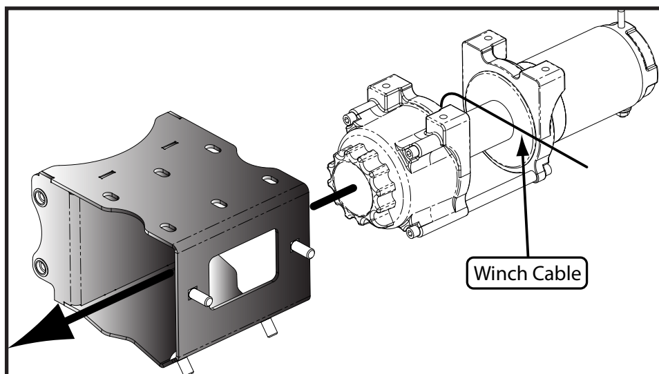
"Figure 3" KFI Winch Install and Position
