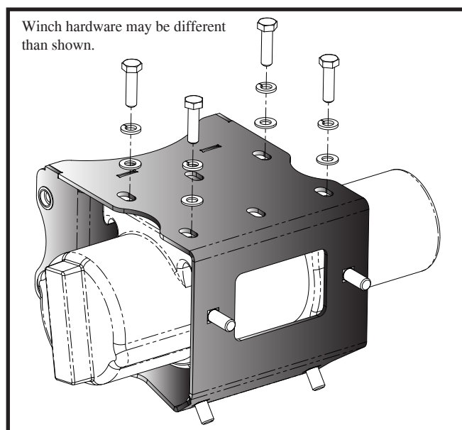
"Figure 8" Winch Bolts Install
