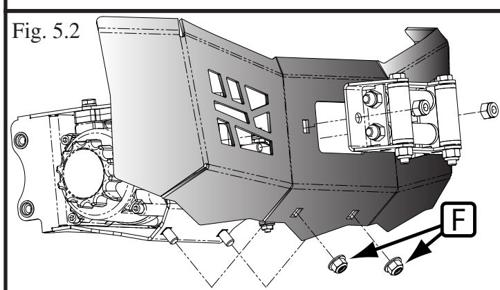
“Figure 5” Guard and Fairlead Install
